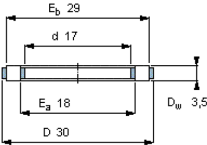
Roller and cage thrust assembly
