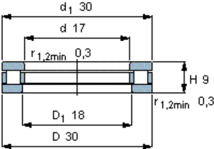
Complete bearing
